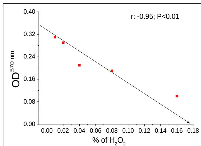
Fig.3 Relationship between biofilm formations in terms of optical density at 570 nm (OD570nm) by K. pneumoniae e (K.p. 3) produced the highest level of biofilm) and the percentages (concentrations) of H 2 O 2 . The negative correlation was seen, r : Pearson correlation coefficient.
