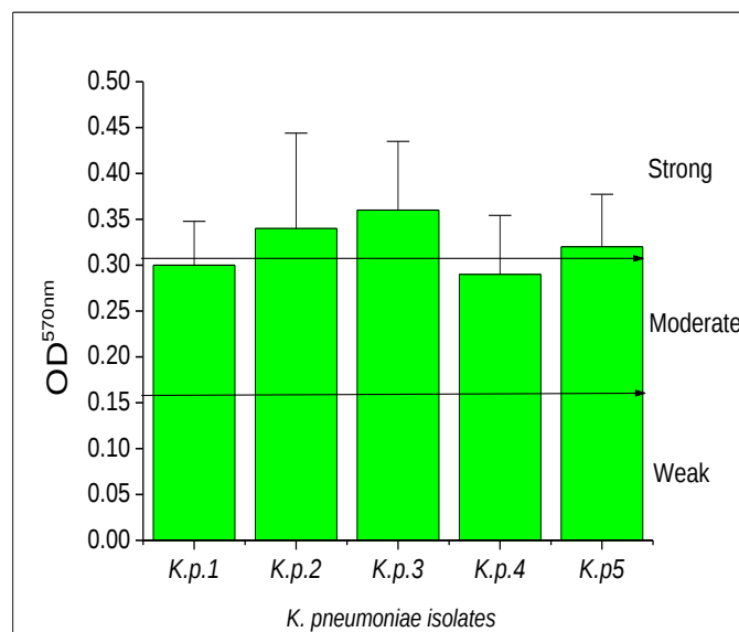
Fig.1 The biofilm formation in terms of the optical density (570nm) of five isolates of K. pneumoniae e that were isolated from urine samples of the patient suffering from UTI. The five isolates were divided into three categories dependent on the level of biofilm formation.
